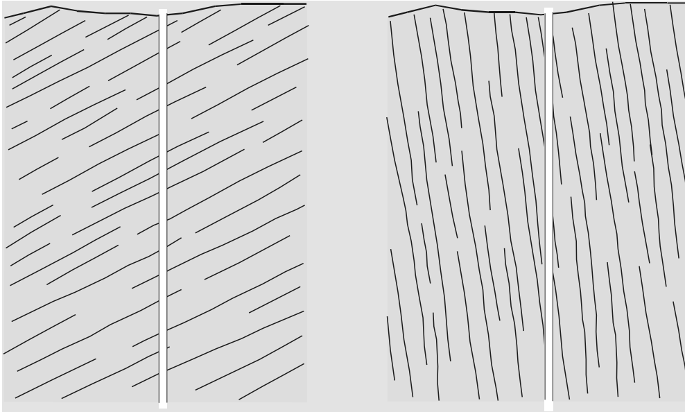
Figure 7 The angle between the main joint set and the bore hole may strongly influence the density of joints along the drill core. The weighted jointing density measurement reduces this source of error
